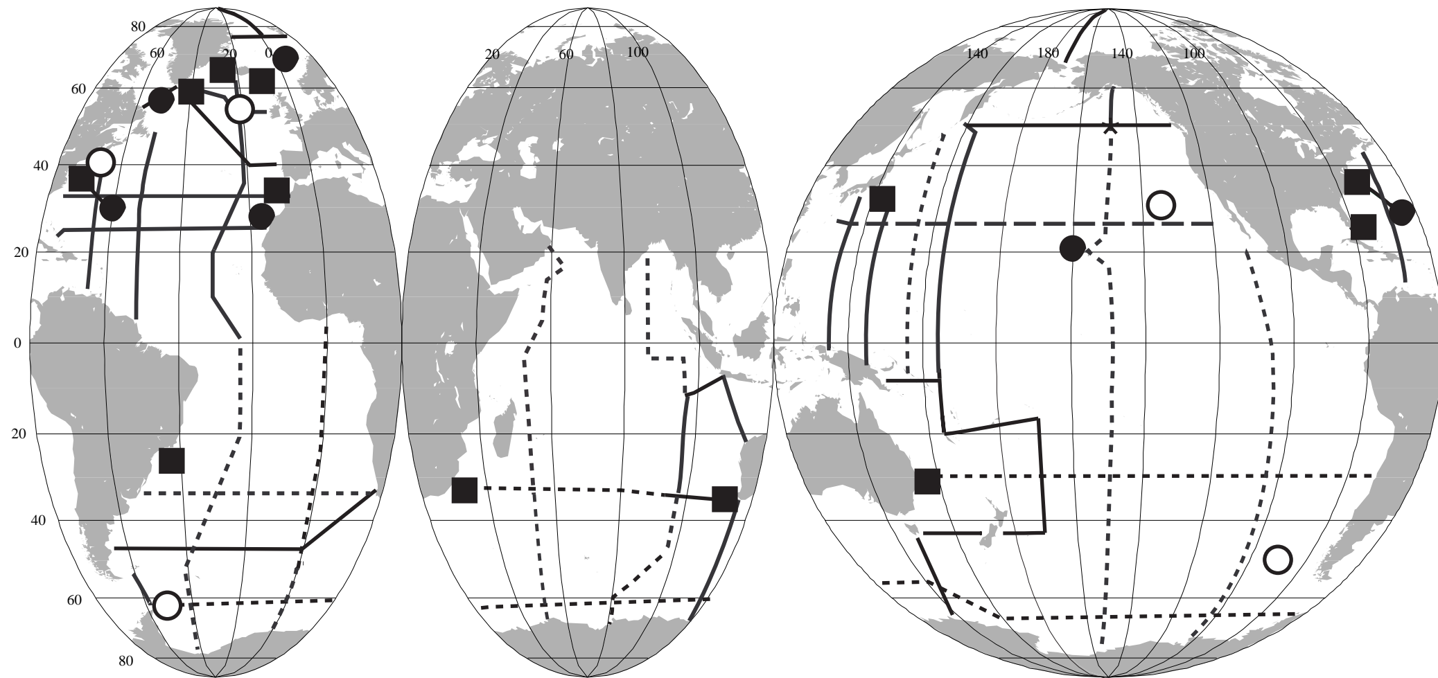
Figure 1. Repeated hydrographic sections and stations recommended for CLIVAR/GOOS. "Committed" sections are already included in national CLIVAR/GOOS plans.
